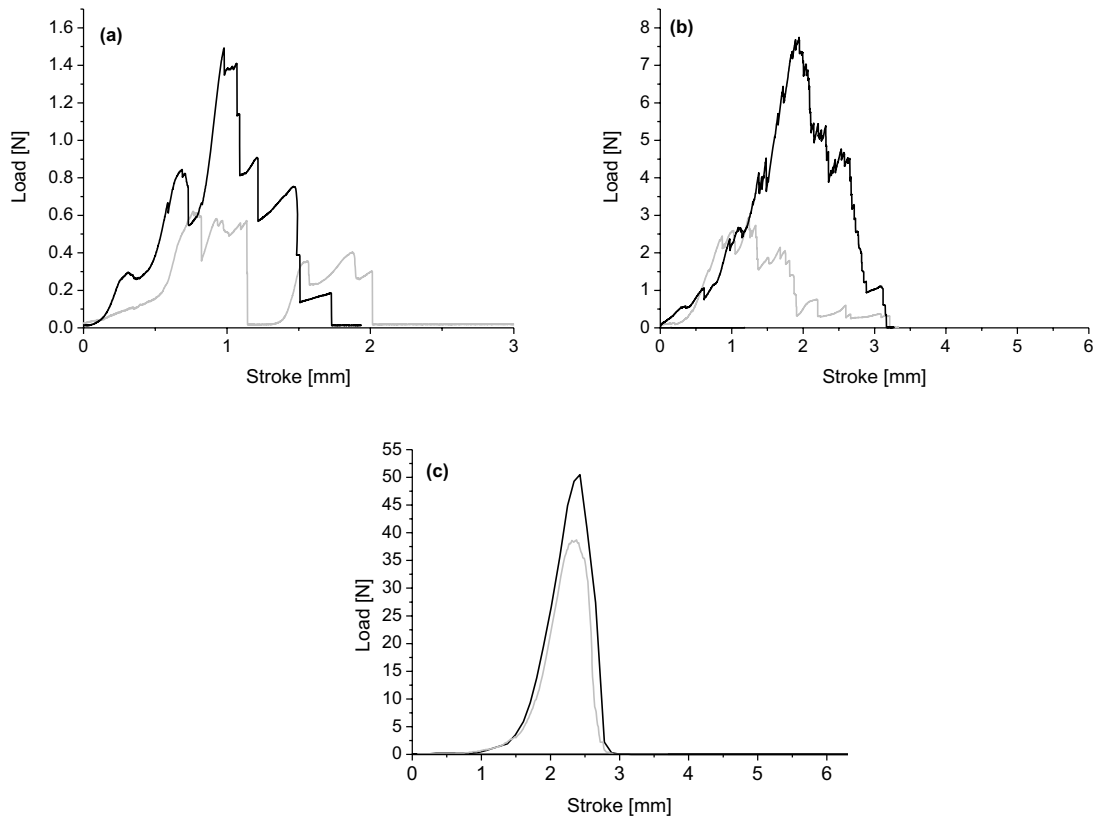
Fig. 3 A diagram of hook load versus stroke for SMA hook arrays with various densities of hooks: (a) 30 hooks/cm 2 , (b) 110 hooks/cm 2 , (c) 240 hooks/cm 2 .
