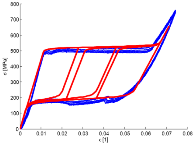
Fig. 4 A diagram of tensile stress-strain curve (a) measured at room temperature for the annealed wire (blue) and (b) modeled tensile stress-strain curve used as an input of the NiTi hook model (red).
