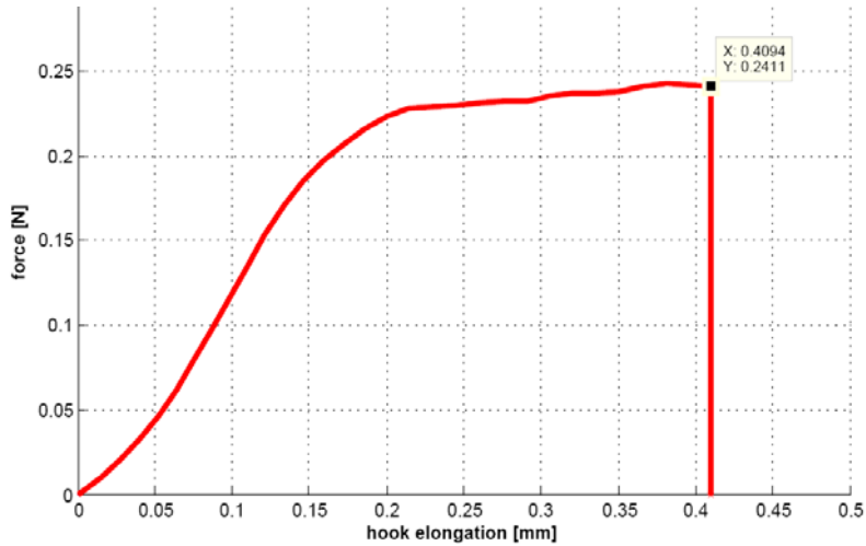
Fig. 6 The diagram of the modeled normal pulling force versus stroke.
