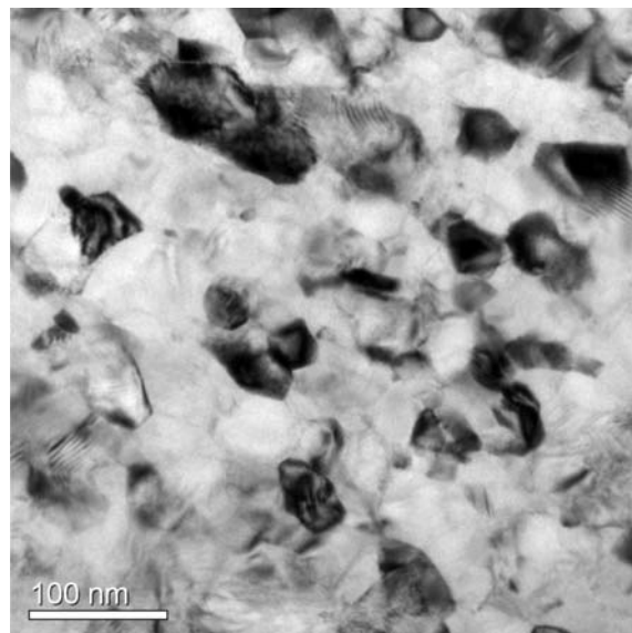
Fig. 3. Microstructure of the NG wire
