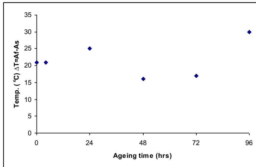
Fig.9 . The temperature differences between the A_f-A_s as a function of ageing time (hrs)
