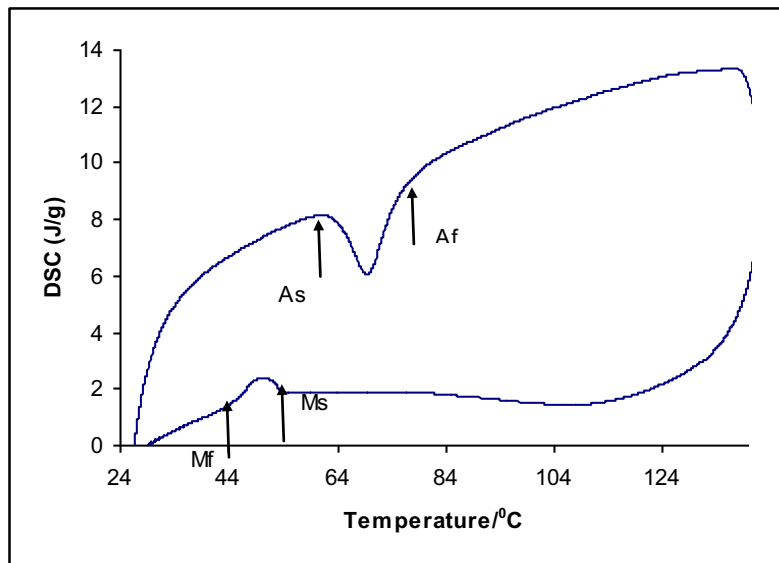
Fig. 2 DSC study of NiTiCu aged sample at 150°C for 4hrs
