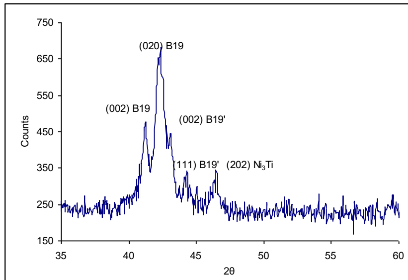
Fig. 7. XRD plot of NiTiCu sample aged at 150°C for 24 hrs exhibiting B19, B19' and Ni 3 Ti precipitates
