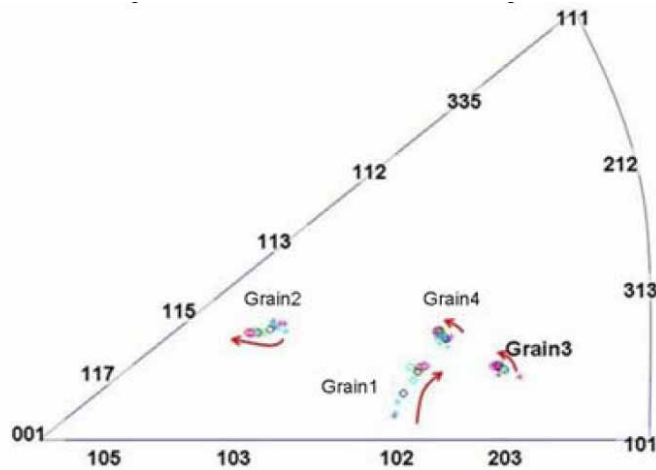
Fig. 4. Inverse pole figure in the tensile direction for the 4 grains.
