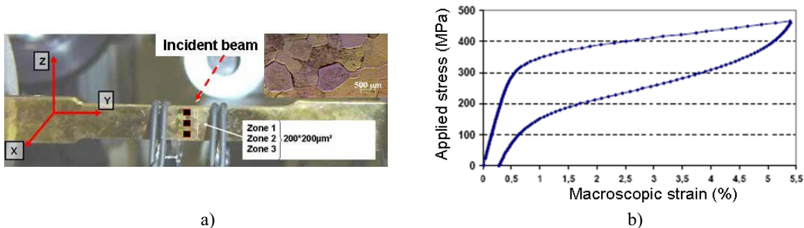
Fig. 2. a) Tensile sample in the tensile rig with the three analysis zones considered. In the upper-left corner: micrograph of the central area showing the grain size. b) Macroscopic stress-strain curve.
