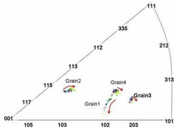
Fig. 3. Inverse pole figure in the tensile direction showing the orientation of the four grains during loading.
