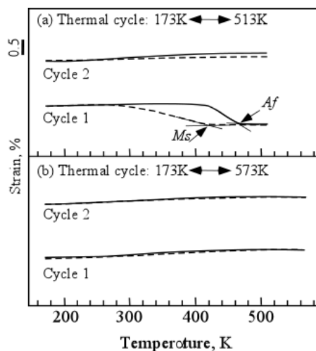
Fig. 3. Thermal cycle tests under a constant stress in Ti-22Nb.
