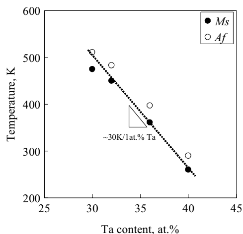
Fig. 1. M_s and A_f temperatures of Ti-Ta solution-treated alloys.
