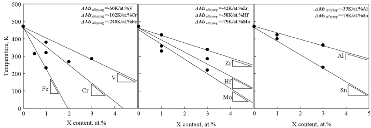
Fig. 7. M_s as a function of alloying content for Ti-30Ta-X alloys.
