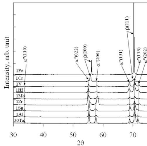
Fig. 5. XRD profiles of Ti-30Ta-1X alloys.
