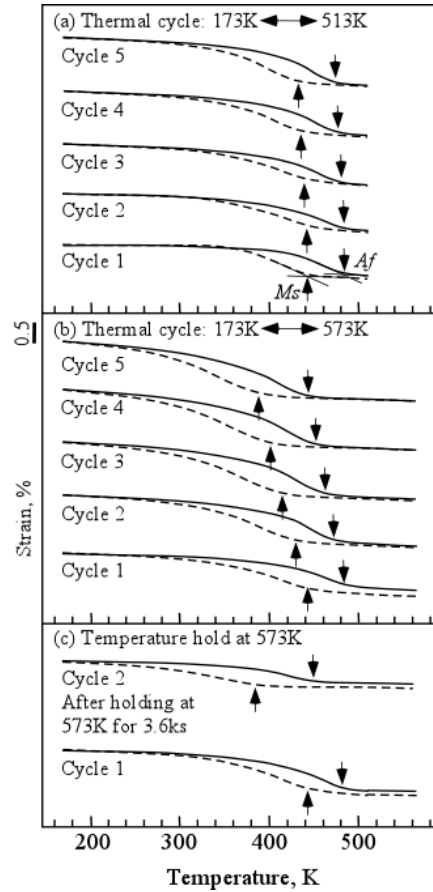
Fig. 2. Thermal cycle tests under a constant stress.
