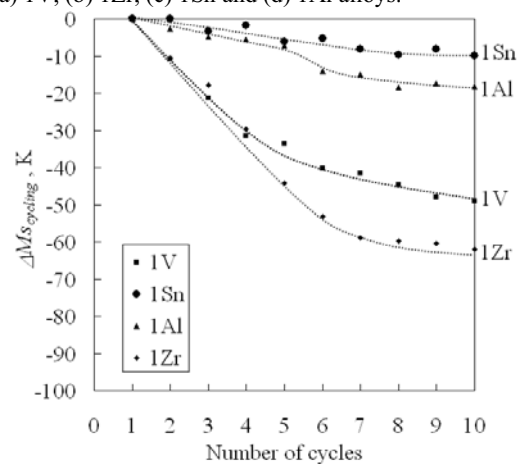
Fig. 10. \Delta M_s vs. the number of cycles for 1Zr, 1Sn and 1Al alloys.
