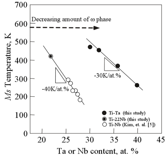
Fig. 4. M_s in Ti-Nb and Ti-Ta alloys.
