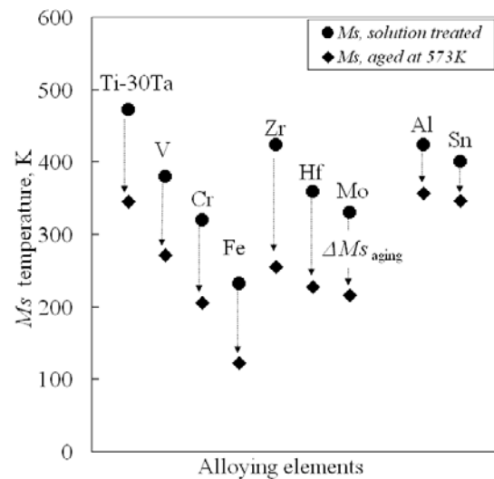
Fig. 8. M_s of Ti-30Ta-X alloys.
