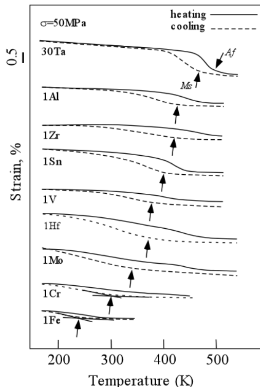
Fig. 6. Strain-temperature curves of Ti-30Ta-1X alloys.
