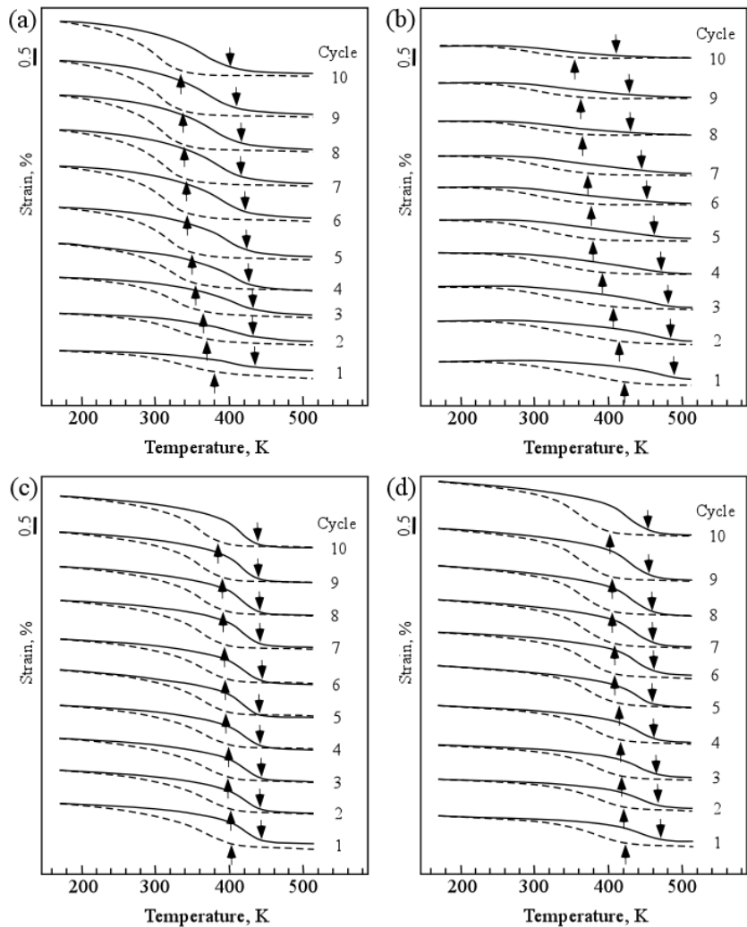
Fig. 9 Strain-temperature curves of (a) 1V, (b) 1Zr, (c) 1Sn and (d) 1Al alloys.
